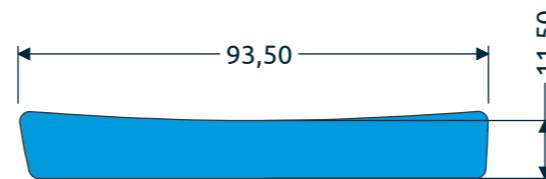
DETAIL B | BOTTOM LOGO SCALE 1 : 1.5
