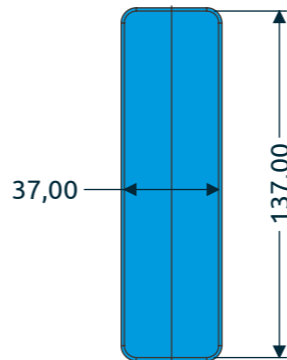
DETAIL B | BACKPLATE LOGO SCALE 1 : 3
