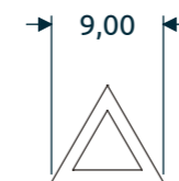
DETAIL A | TACTILE WARNING SCALE 1.5 : 1
